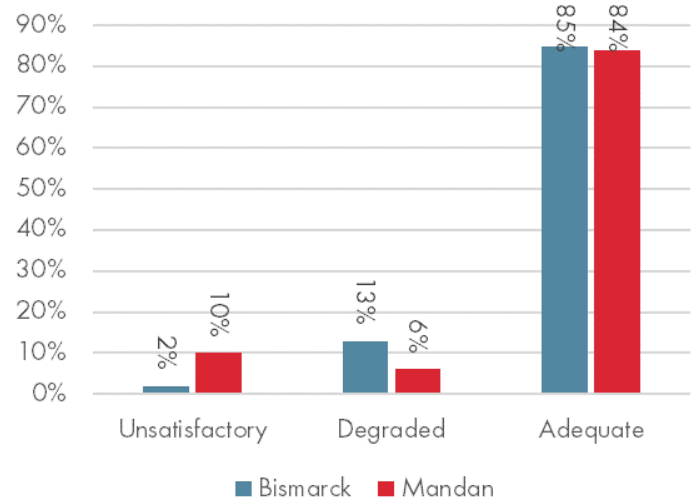
Figure 4.9: PCI Assessment for Bismarck and Mandan
